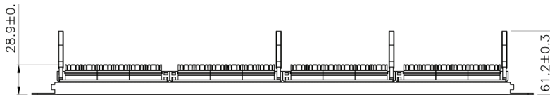
1U 24 Port LSA Block Cat 5E Panel 19" UTP
