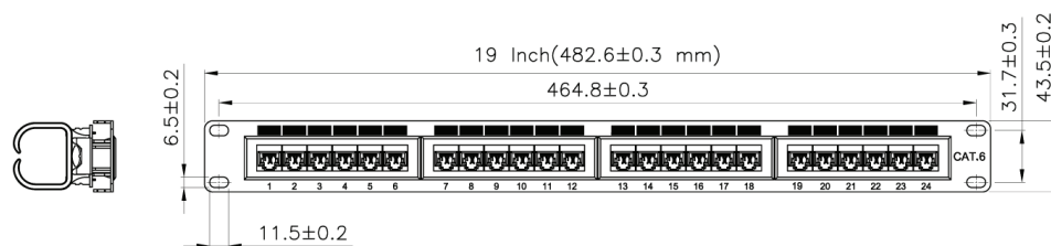
1U 24 Port LSA Block Cat 6 Panel 19" UTP
