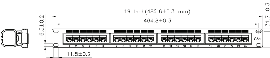
1U 24 Port LSA Block Cat 5E Panel 19" UTP
