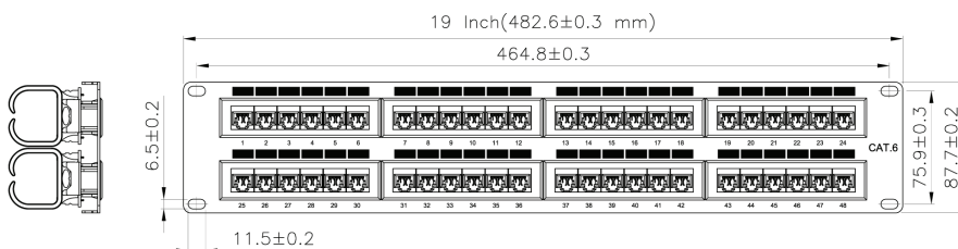
2U 48 Port LSA Block Cat 6 Panel 19" UTP
