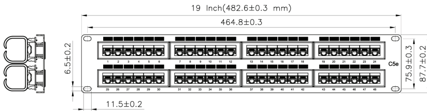
2U 48 Port LSA Block Cat 5E Panel 19" UTP
