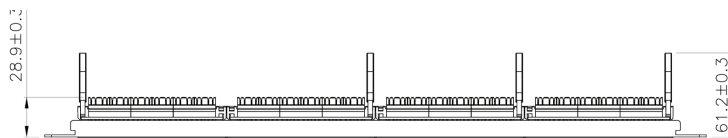
2U 48 Port LSA Block Cat 5E Panel 19" UTP
